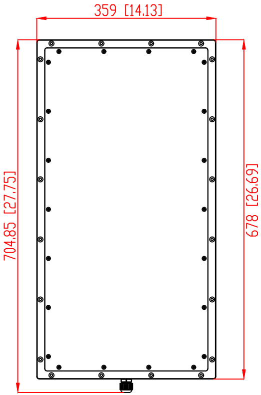
BOTTOM VIEW
