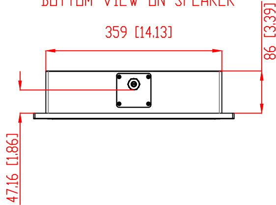
BOTTOM VIEW ON SPEAKER
