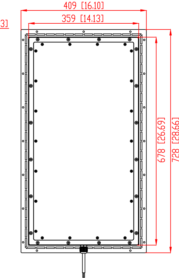
BOTTOM VIEW ON SPEAKER
